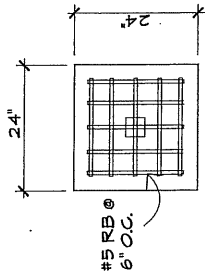
PLAN VIEW
